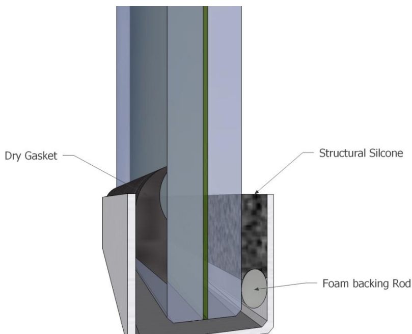
Figure 7 – Base channel, showing two fixing arrangement options – the dry gasket and the structural silicone
