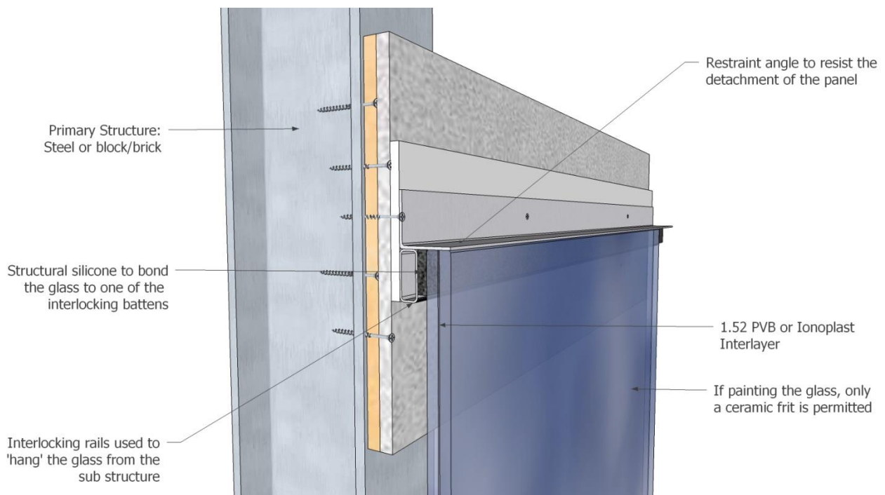
Figure 6 - Glass wall lining, typical detail
