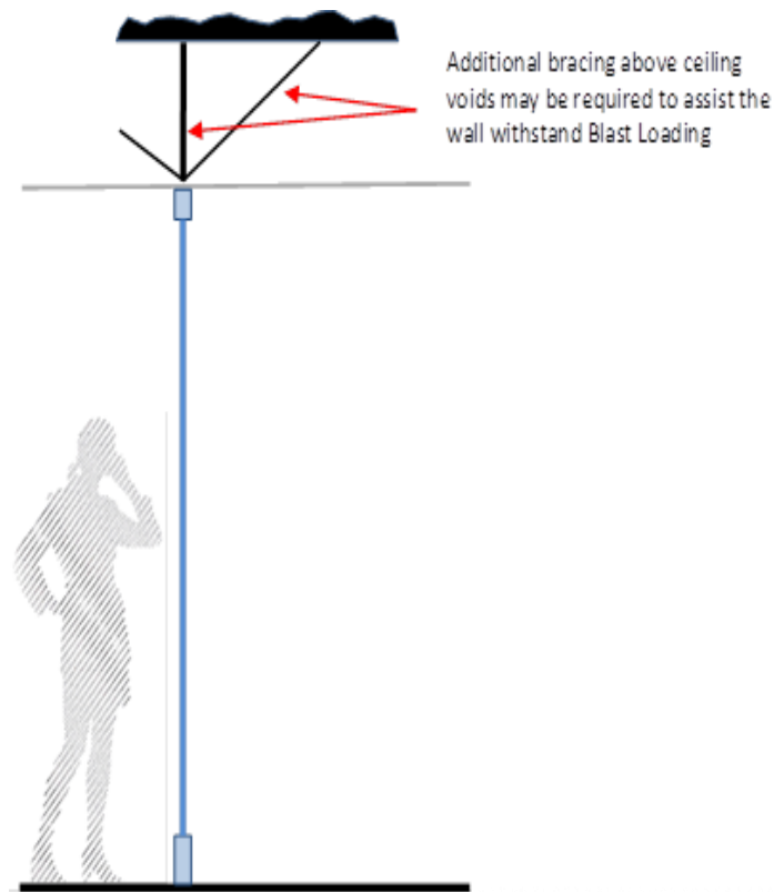
Figure 5 – Glass partition fixing details
